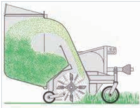
Hydraulic ground level tip on all 'C' models
