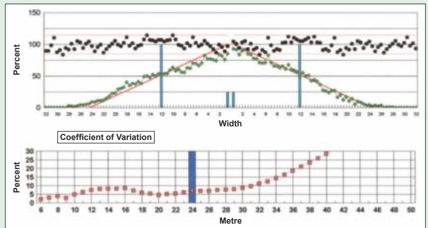
Working width: 24 m, coefficient of variation (VK): 6.9%, fertilizer: CAN
