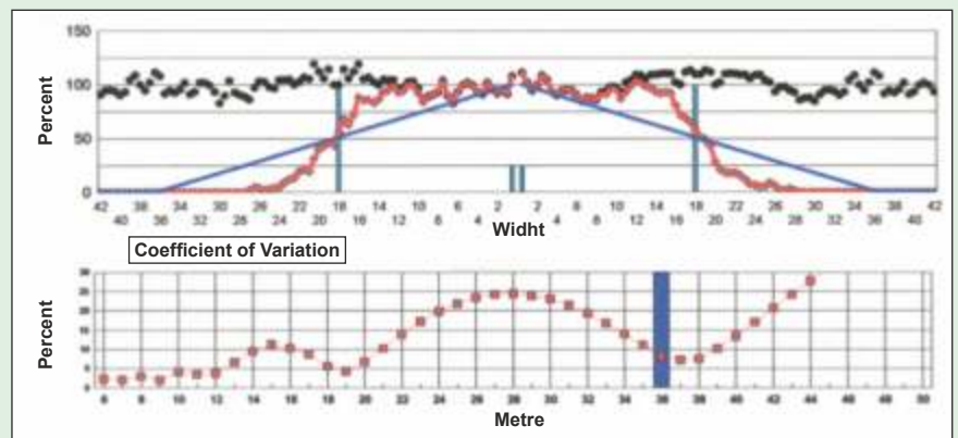
Working width: 36 m, coefficient of variation (VK): 8.25%, fertilizer: NPK
